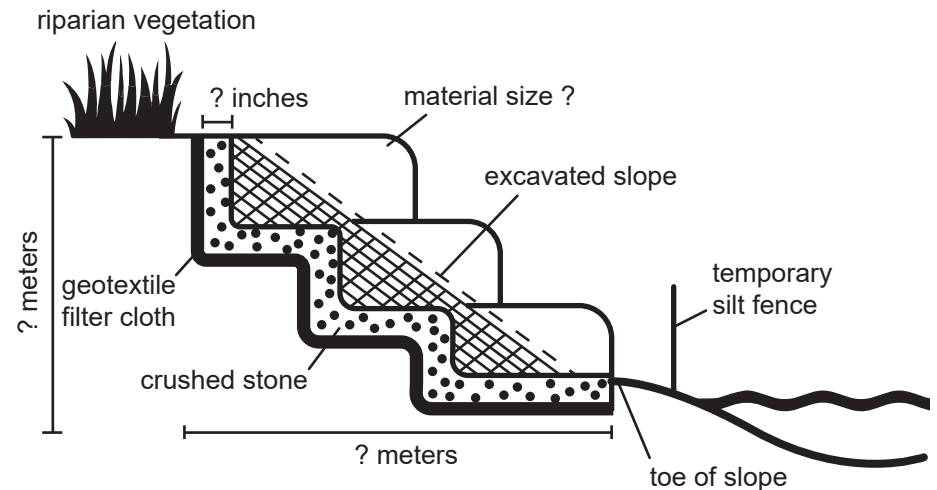
Example # 2 - proposed tiered armour stone wall
