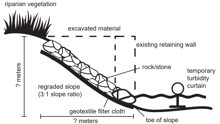
Example # 1 - proposed sloped rock protection
