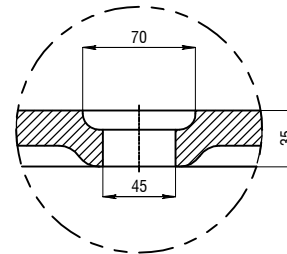
DETAIL D SCALE 1:2
