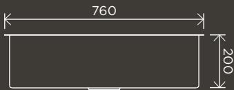
Kitchen Sink - Single Bowl 760 x 440 x 200
