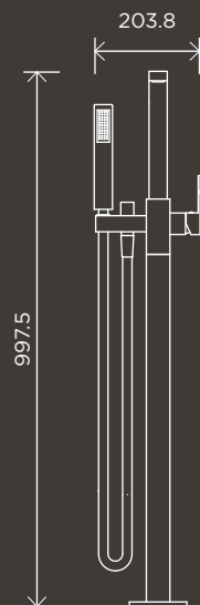
Square Freestanding Bath Spout and Hand Shower
