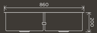
Kitchen Sink - Double Bowl 860 x 440
