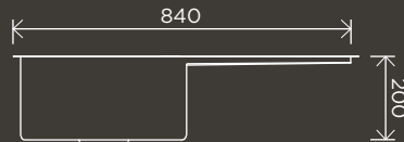
Kitchen Sink - Drainboard Single Bowl 840 x 440 x 200
