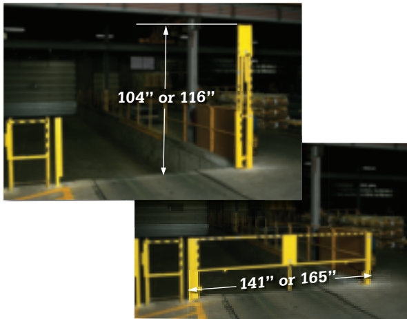
Installation Dimensions
