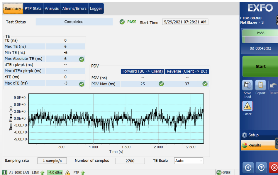
Figure 3. EXFO's Time Error/Wander validates timing accuracy at critical locations in the network.
