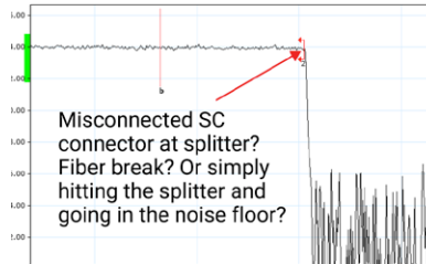
Figure 2. Last-Mile OTDR trace.
