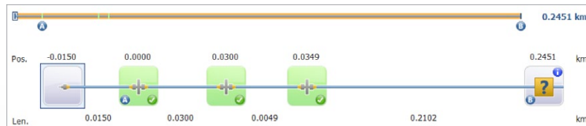
Figure 3. Test fail—Expected splitter not detected. Last mile looks OK but there is either a break or disconnection at splitter.
