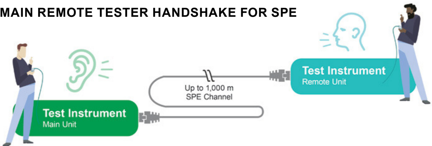
FIGURE 7: One of the challenges in testing SPE cables is the long reach and how the attenuation or insertion loss causes the signal to decay as the length of the cable increases. 3
