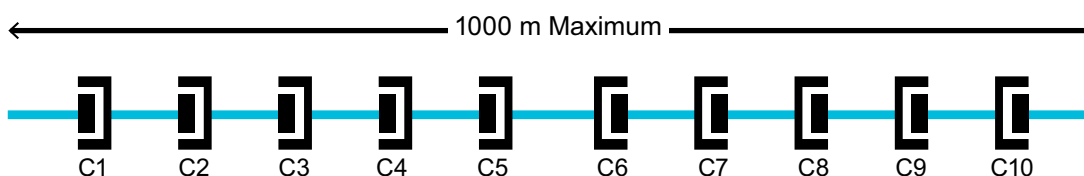
FIGURE 2: Single-pair Ethernet Topologies.
