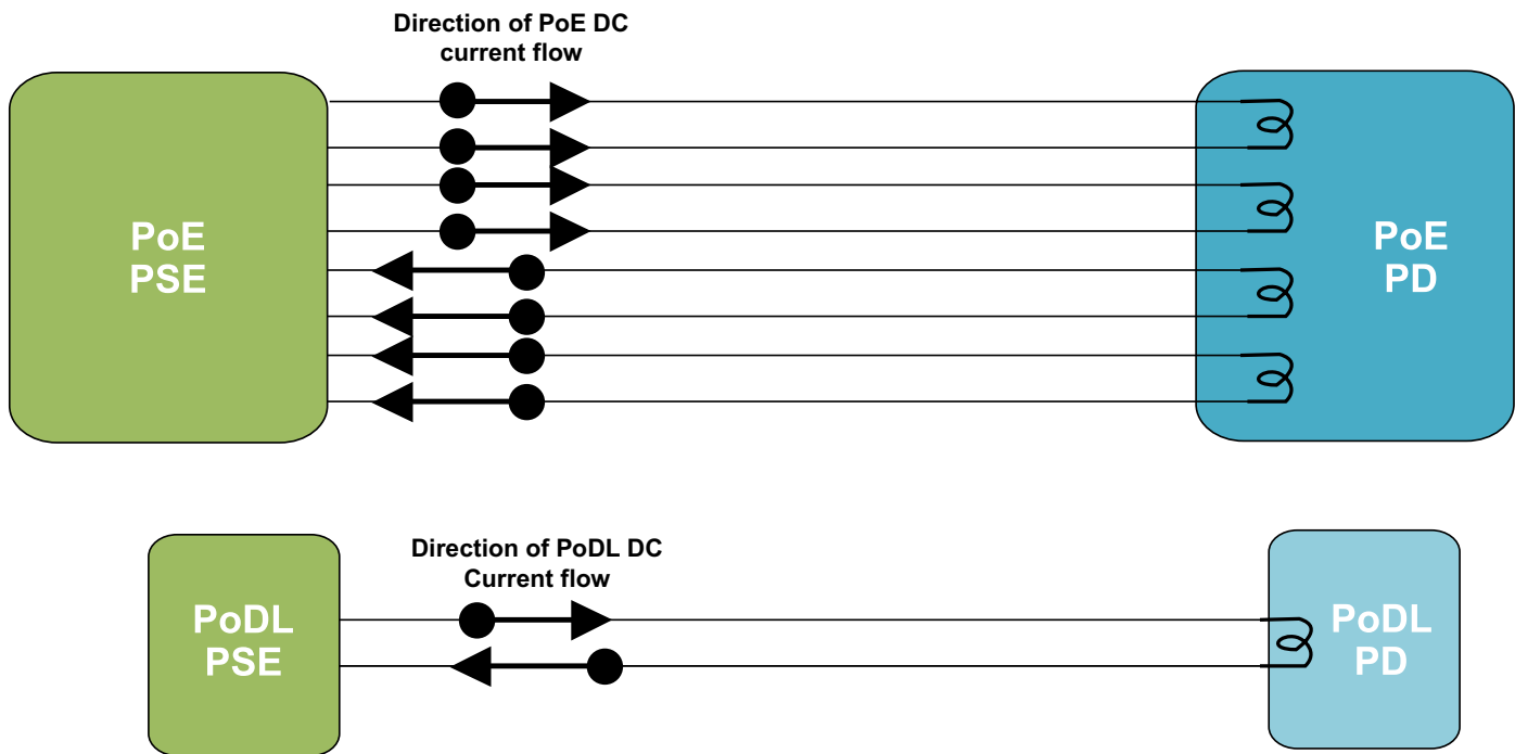
FIGURE 9: Direction of current flow for 4-pair cabling versus SPE. Top: 4-pair solution. Bottom illustration: SPE. PSE is defined as power source equipment.
