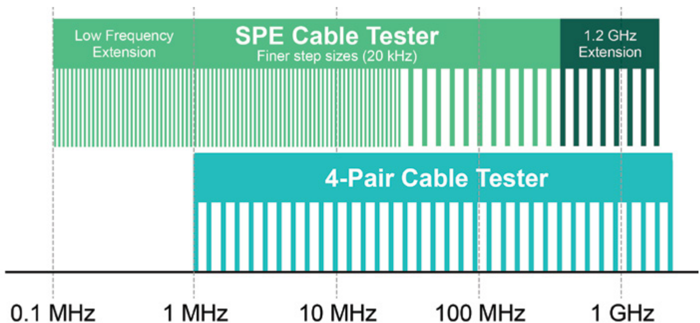
FIGURE 8: Testers for SPE will need to support finer frequency step resolution compared to 4-pair systems.
