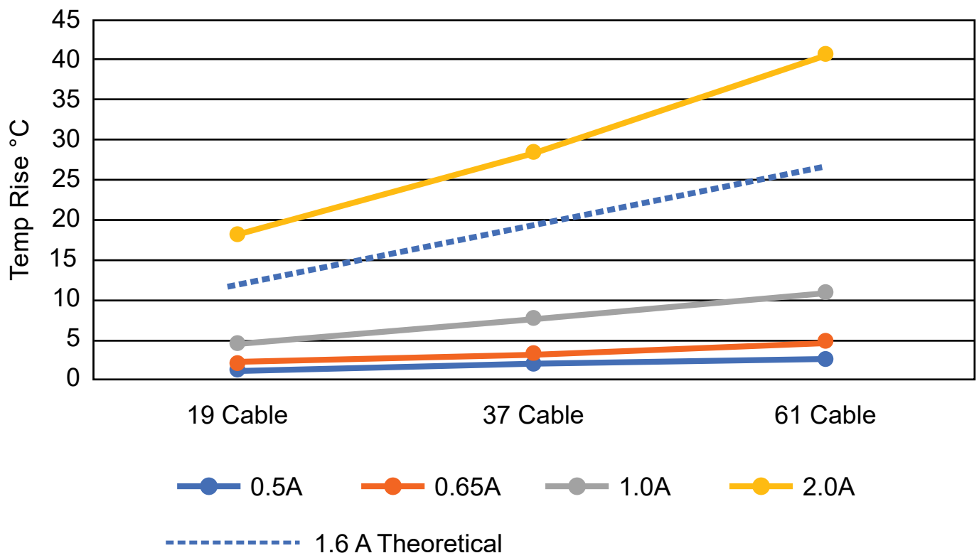
FIGURE 4: Temperature rise versus bundled cable size.
