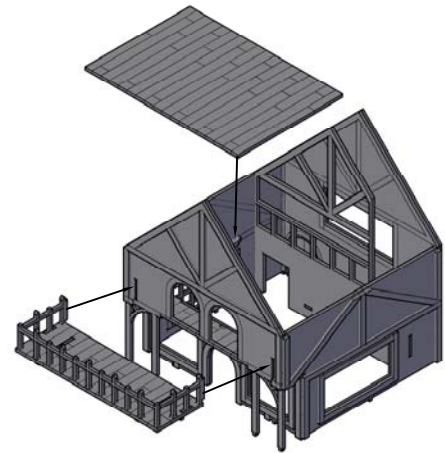
STEP:02 - GLUE TOGETHER WALLS
