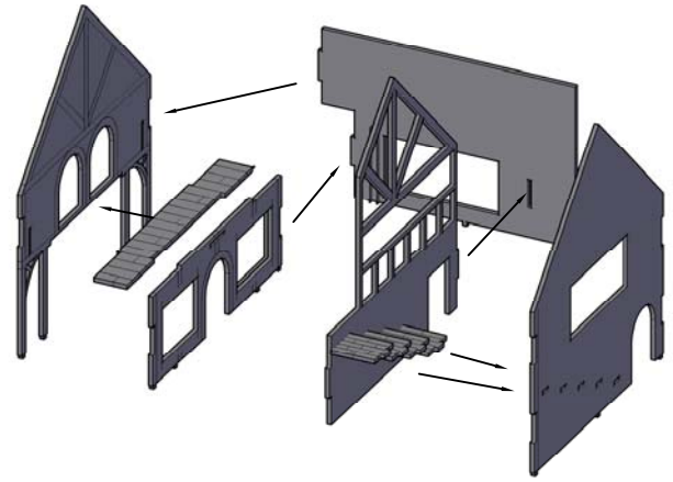
STEP:02 - GLUE TOGETHER WALLS
