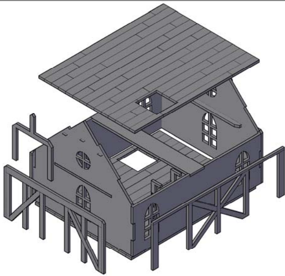
STEP:07 – SIDE MOLDING IS OPTIONAL AND FLOOR IS LEFT MODULAR
