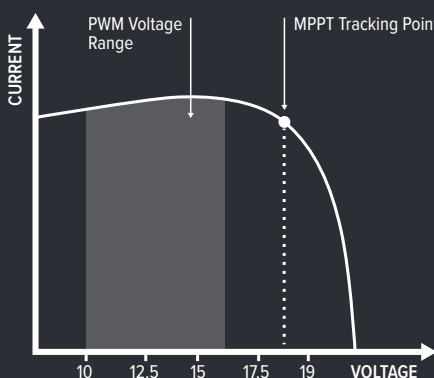
MAXIMUM POWER POINT TRACKING (MPPT)
