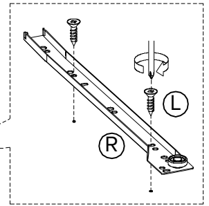
SECTION B
