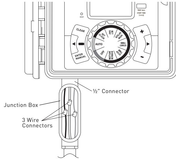
Figure 5: Using a Junction Box
