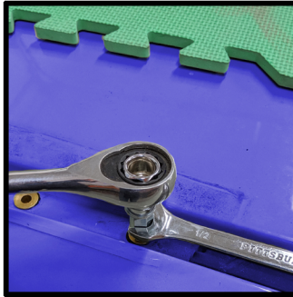
Compress the plusnut by using a 1/2" wrench to hold the coupler and tighten with a 7/16" wrench
