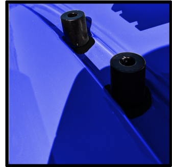
Apply more silicone over the plusnuts before placing the spacers down to ensure a water tight seal
