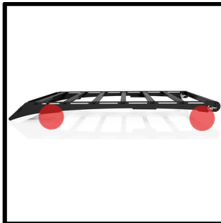
Place the 5/8" spacers under the front and the back mounting feet
