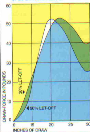
Compound Bow Draw-Force Curve Showing Comparison of 30 and 50% Let-off
