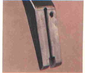
B. The back of each limb is machined with a locator pinhole and limb microgroove alignment key way. The locator pin and pinhole match for perfect fit and positive limb alignment.
