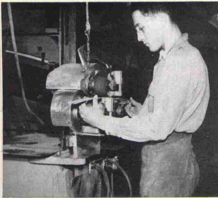
Adhesive is mechanically applied to laminates. In this plant, most of the machines are Bear-designed and Bear-constructed.
