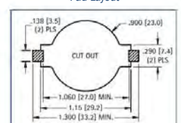
Pad Layout
