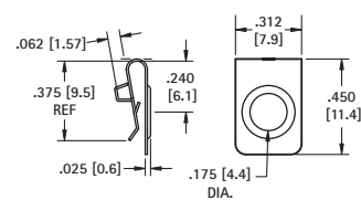
MATERIAL: 010 (.25) Spring Steel, Nickel Plate
