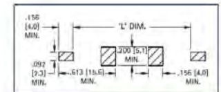
Pad Layout
