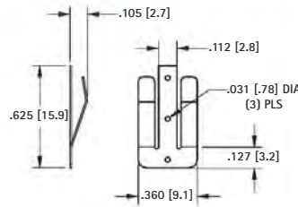
SMT SPRING CONTACT*
