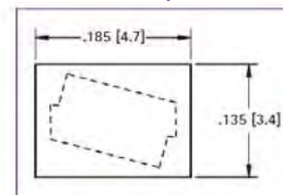
Pad Layout
