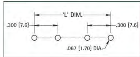
Mounting Detail
