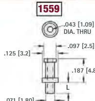
Staking Tool No. TL-2
