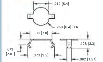
Mounting Detail
