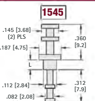
Staking Tool No. TL-12
