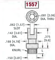
Staking Tool 1557-TL
