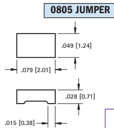
Mounting Detail
