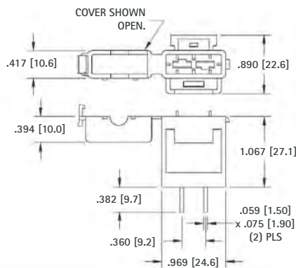
Mounting Detail
