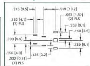
Mounting Detail For Two Holders
