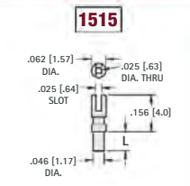
Staking Tool 1515-TL
