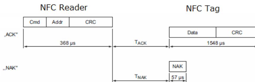
Figure 29 – NFC read command sequence
