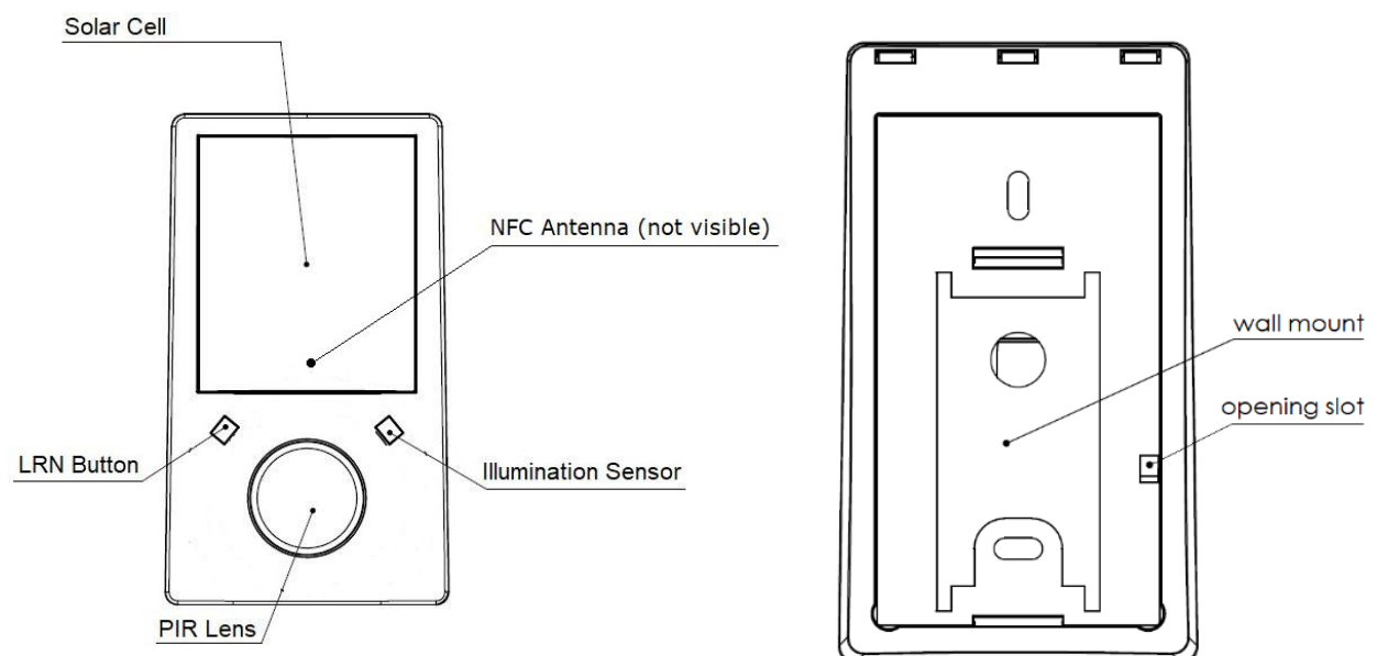
Figure 2 – EMDCB front and rear view
