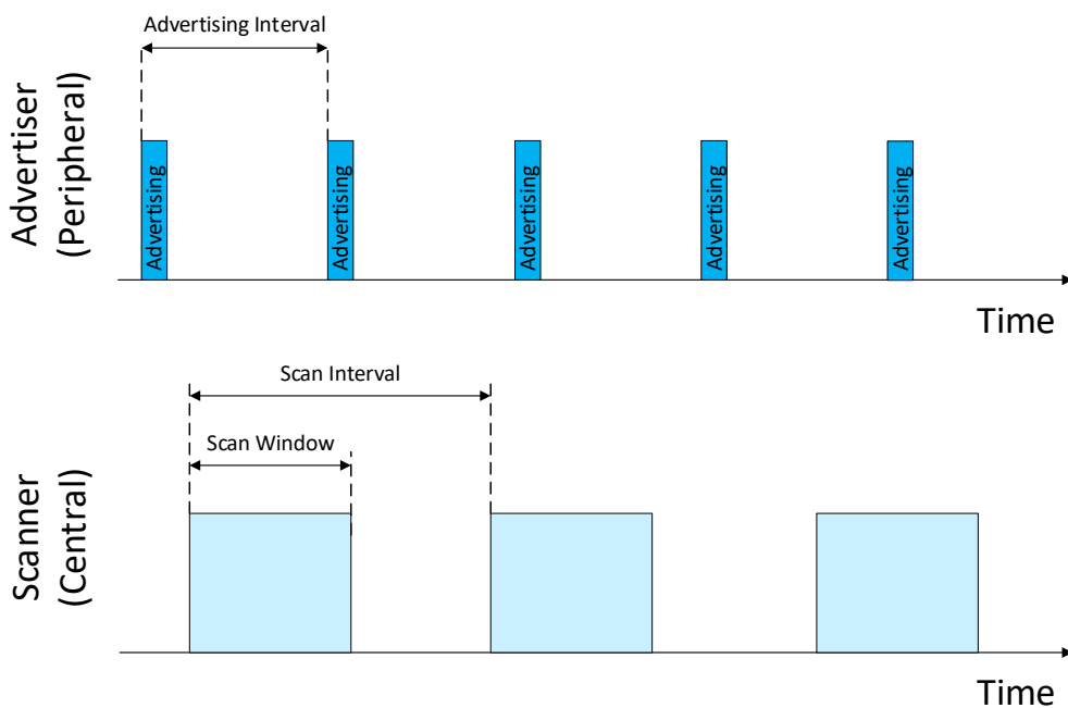
Figure 50 – Scanning parameters
