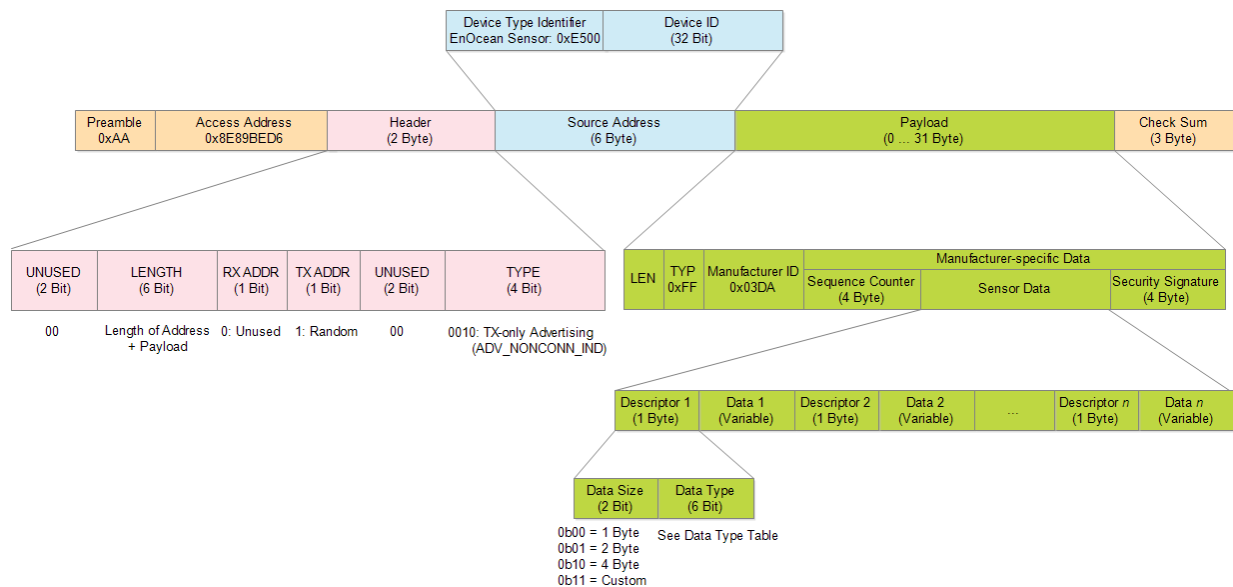
Figure 15 – BLE frame structure
