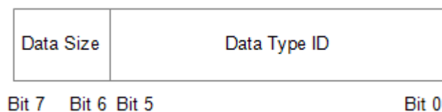
Figure 22 – Sensor Data Descriptor field structure
