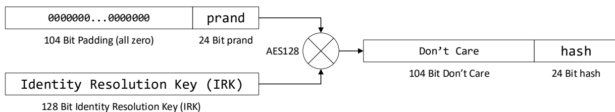
Figure 54 – Execution flow for resolving private addresses (RPA resolution)
