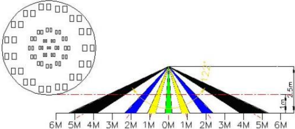
Figure 7 – EMDCB PIR detection pattern
