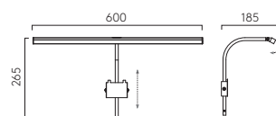
MONDRIAN FRAME MOUNTED 600
