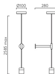
PENDANT SUSPENSION KIT 3 / KNURLED
