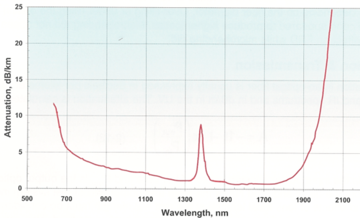
Figure 2-18 Attenuation, Type FI - Low -OH
