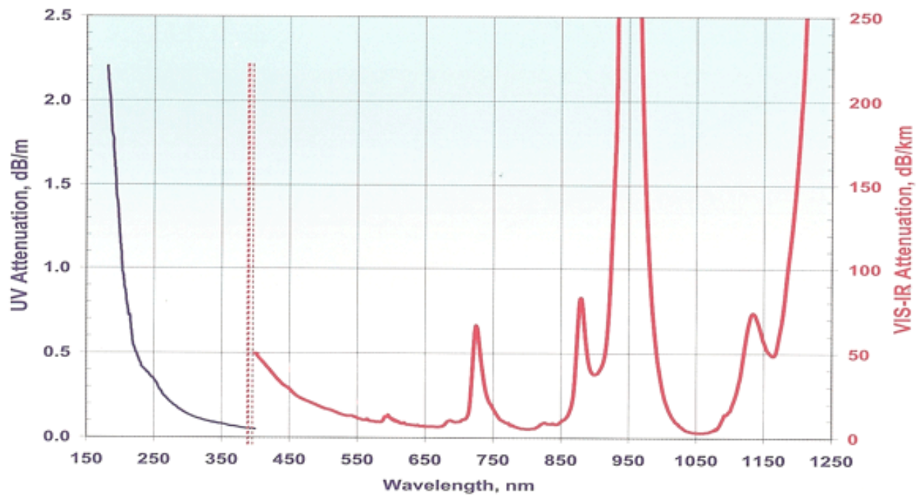
Figure 2-19 Attenuation, Type FV - High -OH
