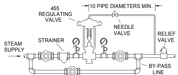
TYPICAL INSTALLATION
