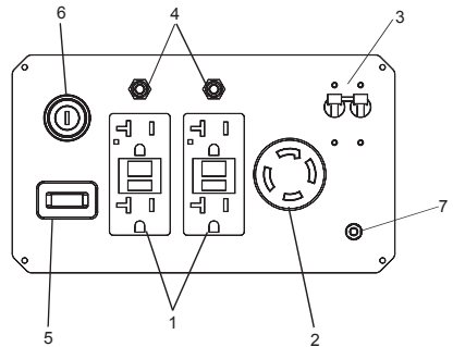
Figure 2-2. Control Panel
