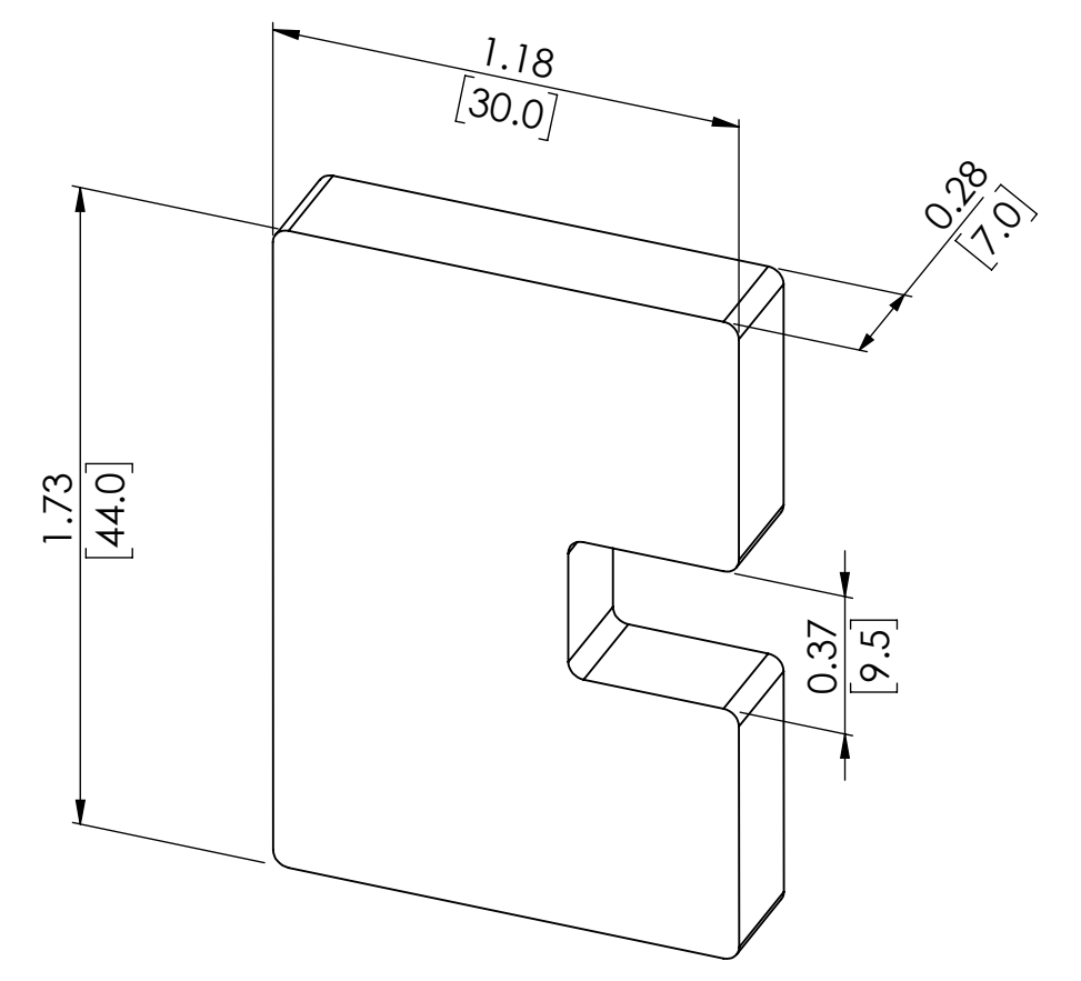
GASKETS FOR 9/16" GLASS
