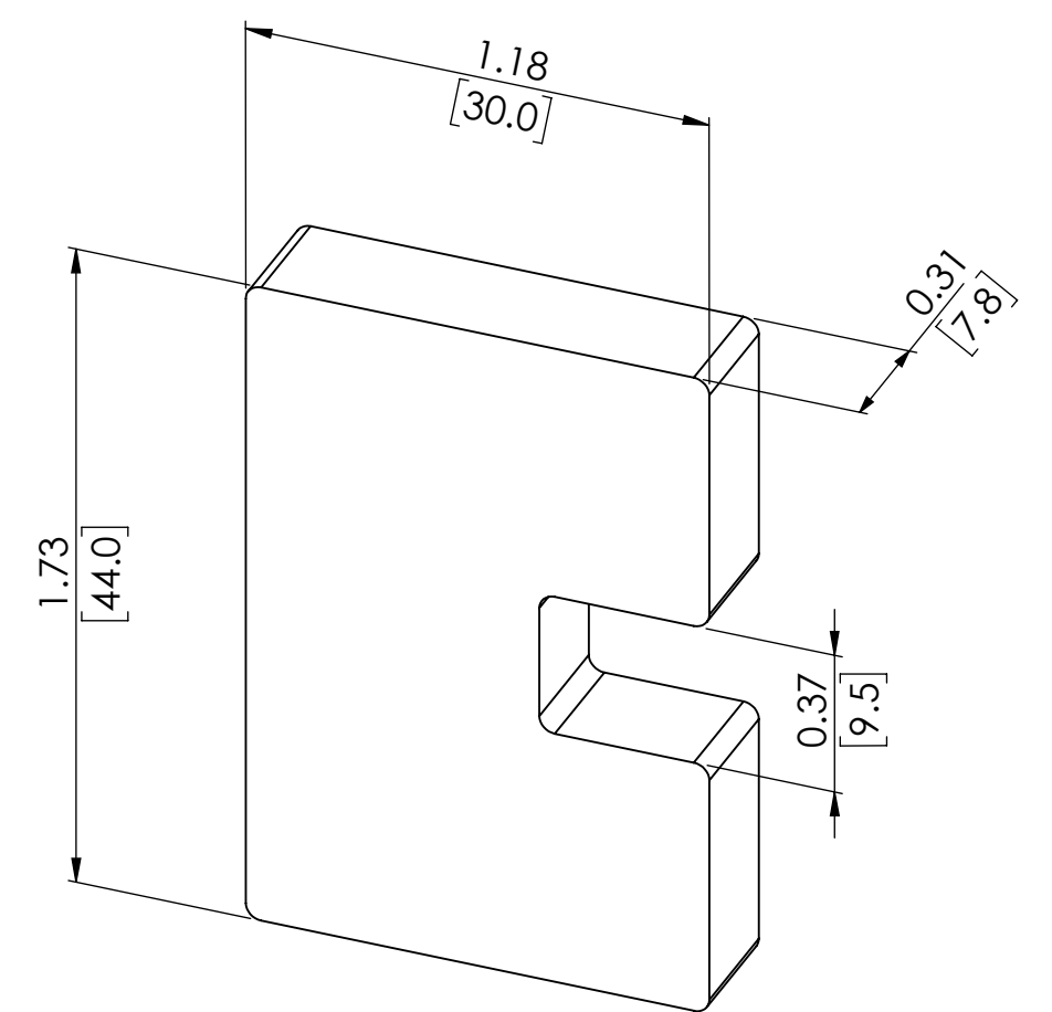
GASKETS FOR 1/2" GLASS
