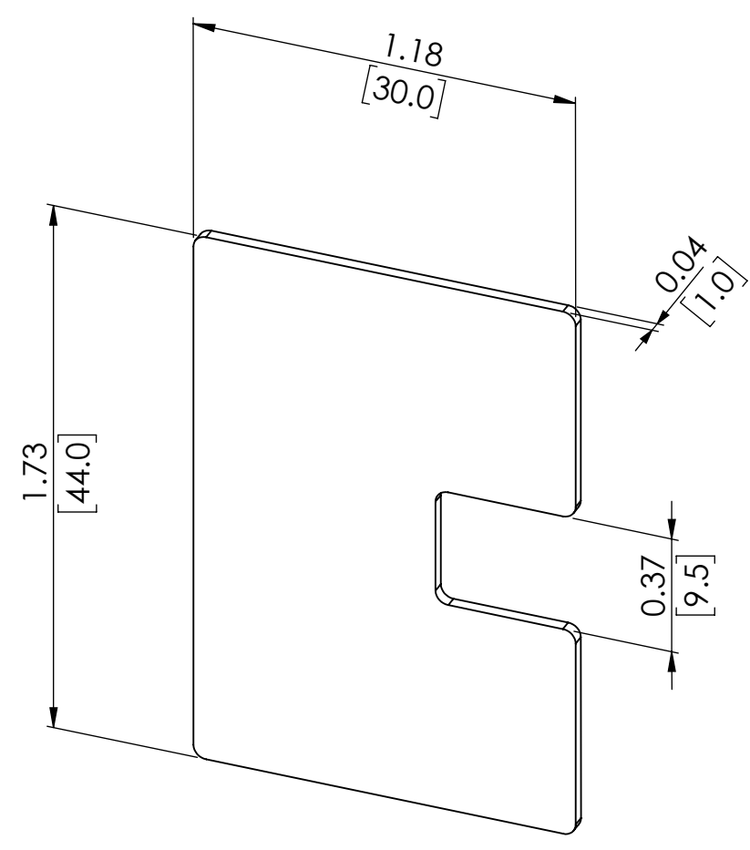
ADD ON GASKETS FOR 3/8" GLASS
