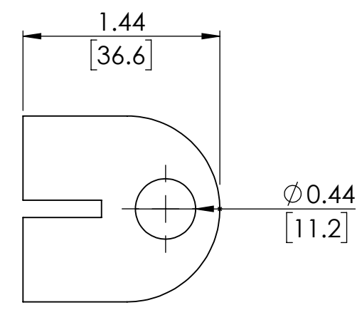
GASKETS FOR 1/2" GLASS
