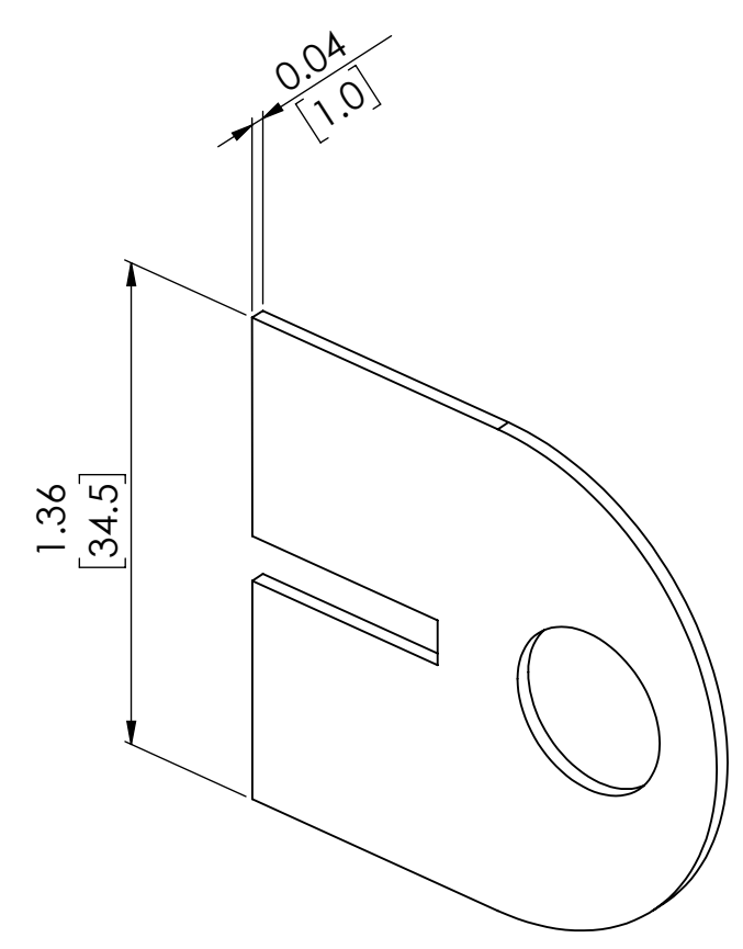
ADD ON GASKETS FOR 3/8" GLASS
