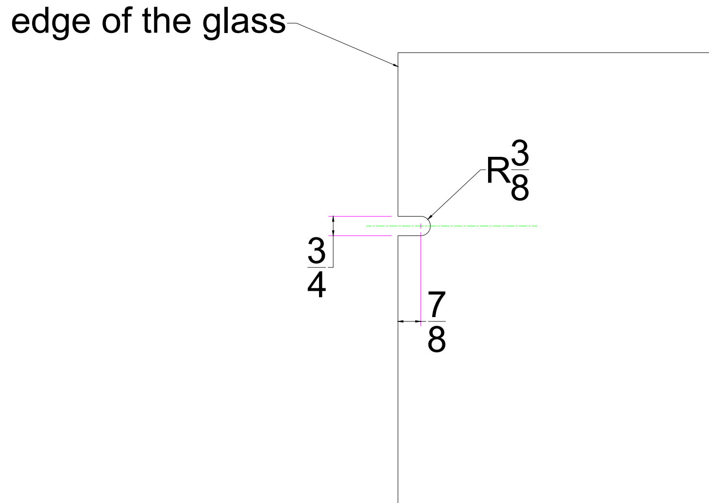
Notch's Dimensions
