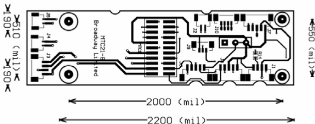
(HO Scale MTC21 motherboard socket)
