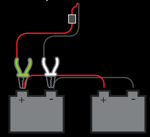
How NOT wire alligator clips for 2 batteries
