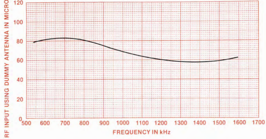
AM MINIMUM USABLE SENSITIVITY (IHF)
