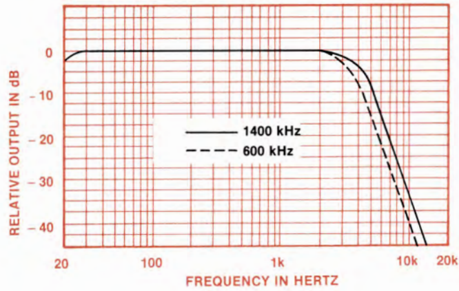
A.M. FREQUENCY RESPONSE 80% Modulation
