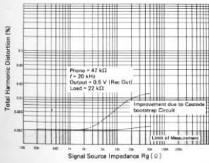
Improvement in Distortion with Cascade-Bootstrap Circuit
