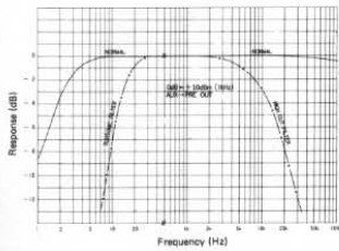
RIAA Deviation (PHONO MM to REC OUT)
