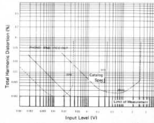
Total Harmonic Distortion vs. Input Level for the MC Head Amplifier (PHONO MC to REC OUT)
