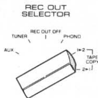
Tape Dubbing (1▶2)
