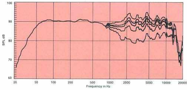
Figure 6. Control Range, Mid
