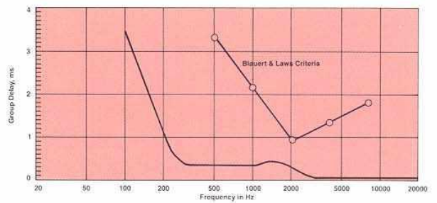
Figure 5. Group Delay vs. Frequency
