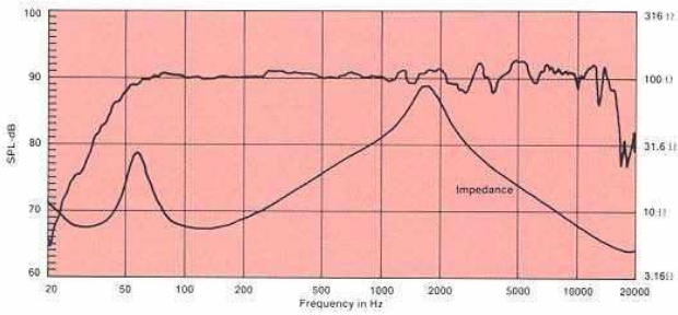
Figure 8. Impedance and On-axis Response
