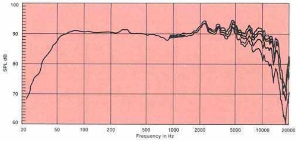
Figure 7. Control Range, High
