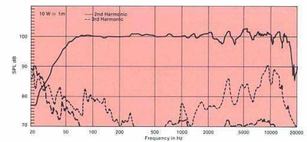
Figure 12. Distortion vs. Frequency
