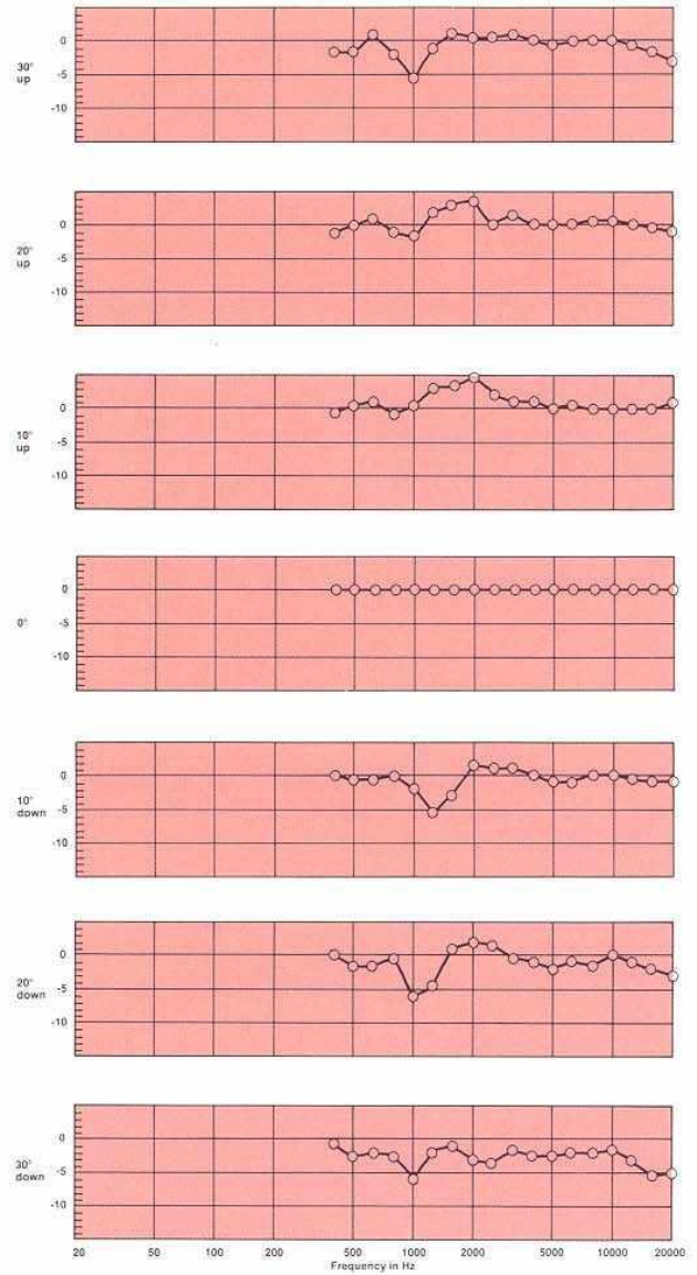
Figure 4. Vertical Off-axis Response (normalized):
