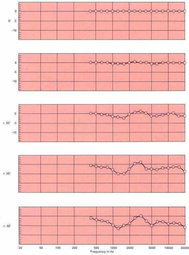
Figure 3. Horizontal Off-axis Response (normalized):
