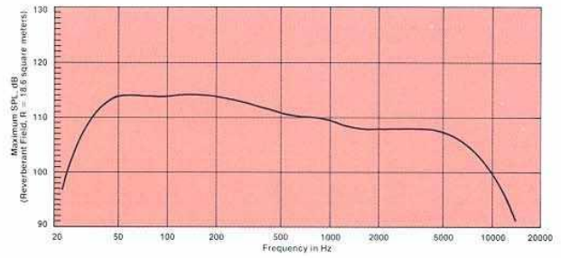
Figure 10. Maximum Continuous Output
