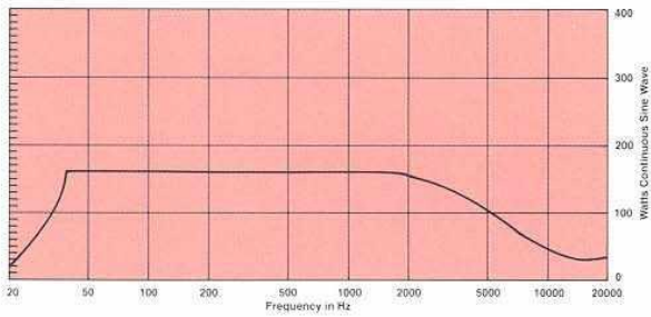
Figure 9. Maximum Electrical Input
