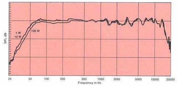
Figure 11. Power Linearity (1 W, 10 W, 100 W)
