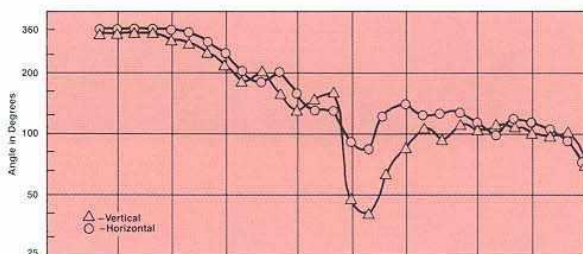
Figure 1. Beamwidth (horizontal and vertical) vs. Frequency
