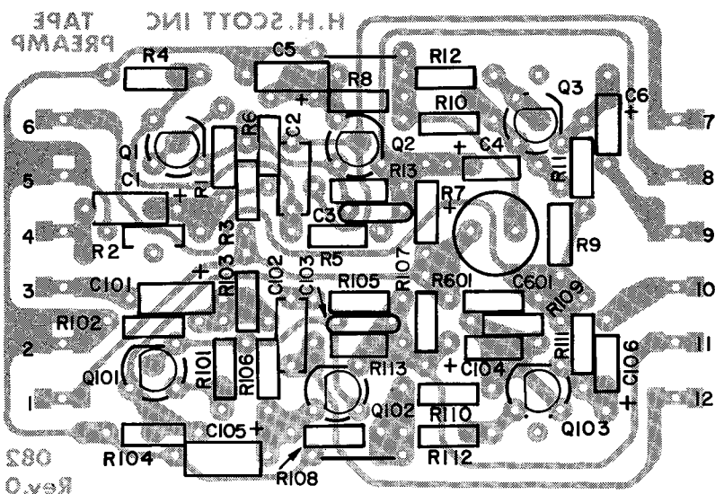
TAPE HEAD PREAMP
