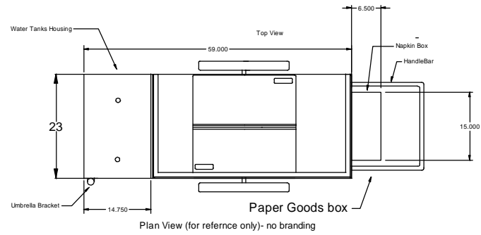
Sizing Template for Turnkey Parlor Custom Non Mechanical Cart- order 1248134
