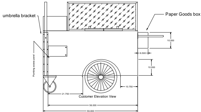
Sizing Template for Turnkey Parlor Custom Non Mechanical Cart- order 1248134
