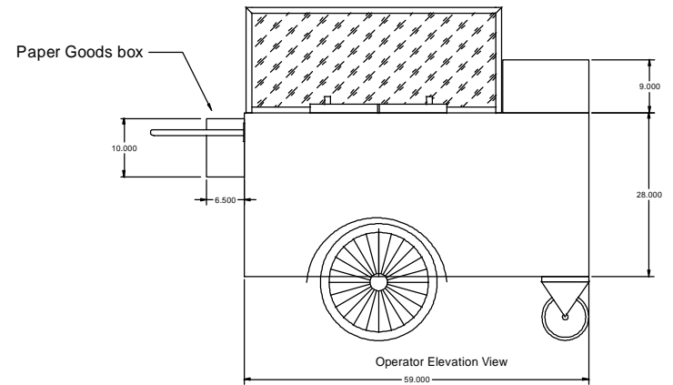
Sizing Template for Turnkey Parlor Custom Non Mechanical Cart- order 1248134
