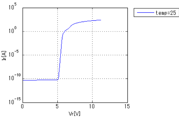
IrVr(Breakdown)
