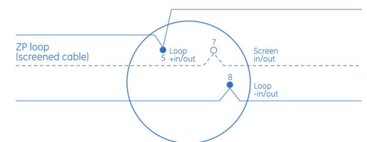
ZP7-SB1 / ZP7-RB1 Sensor base
