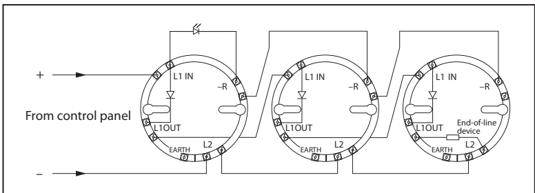
Wiring Diagram of Series 65 Monitored Detector Circuit with a common Remote Indicator
