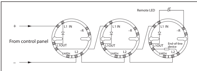
Wiring Diagram of Series 65 Monitored Detector Circuit
