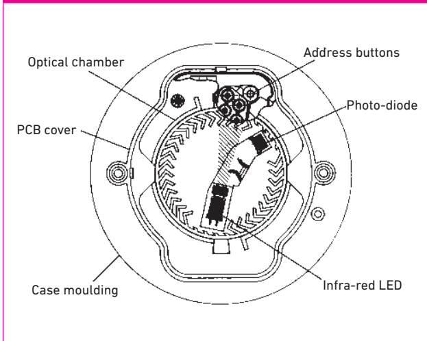
XP95 Optical Smoke Detector sectional view
