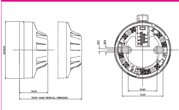
XP95 Optical Smoke Detector dimensions
