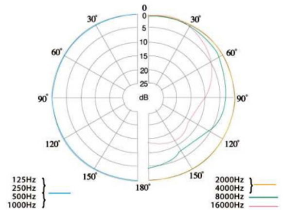
TYPICAL POLAR PATTERN
