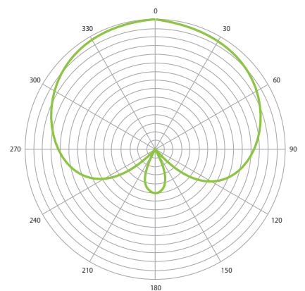
TYPICAL POLAR PATTERN FIGURE 2
