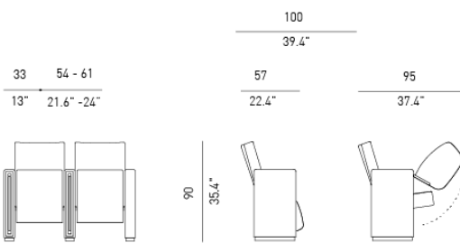
Flex 6076 + A3PL
