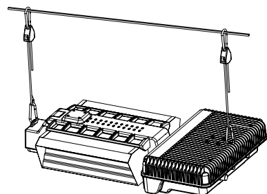
Intermediate sling installation
