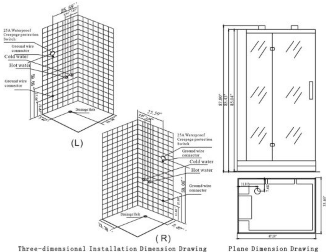
Three-dimensional Installation Dimension Drawing
