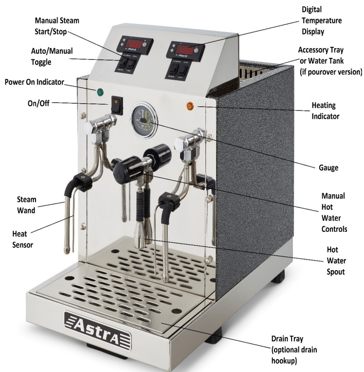
FIGURE 2: SEMI-AUTOMATIC STEAMER
