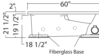
10-jet Bodywrap System SB-3660 BWS (illustrated)
