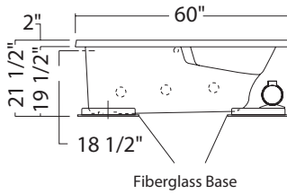
6-jet Homestead Collection SB-3660 HMS (illustrated)
