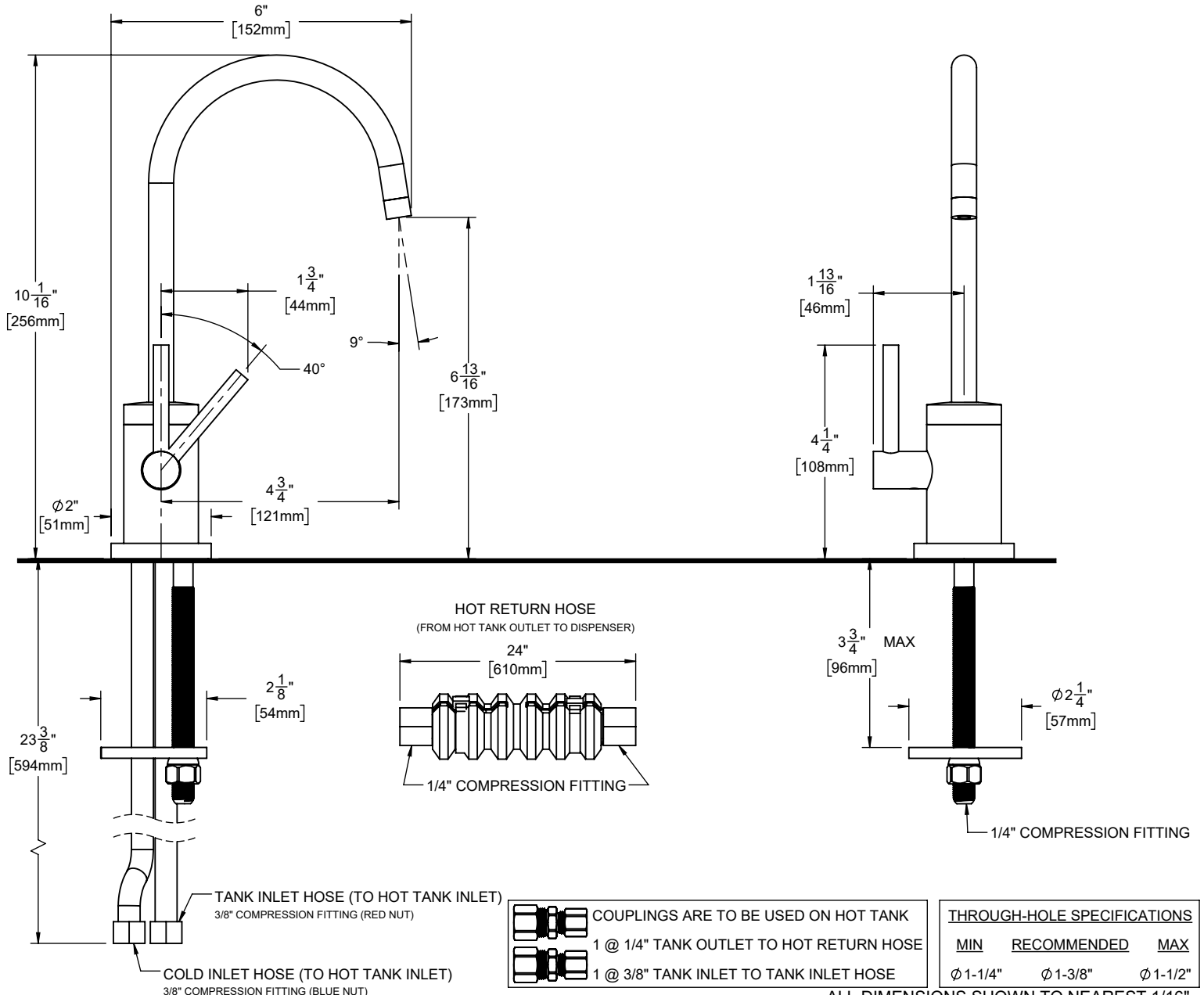
9625-K50-ST shown
