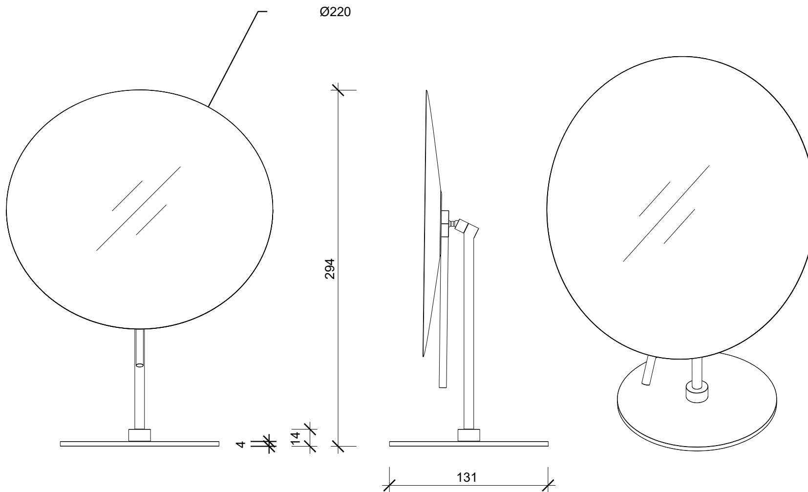
Frontansicht front view
