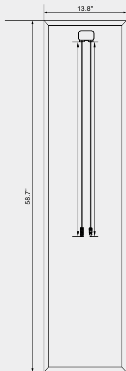
Back Profile (unit: inch)
