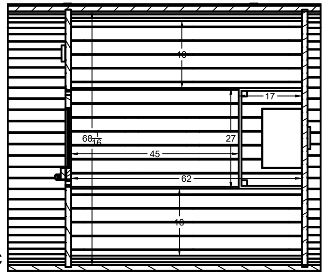
SECTION C-C SCALE 1:25
