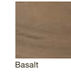
Basalt
