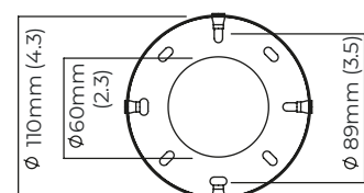
mounting plate dimensions
