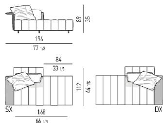
ELEMENTO TERMINALE PENISOLA CM 196 - SCHIENALE CM 84 OPEN-END ELEMENT WITH ARMREST CM 196 - BACKREST CM 84
