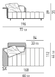
ELEMENTO TERMINALE PENISOLA CM 196 - SCHIENALE "WING" CM 84 OPEN-END ELEMENT WITH 1 ARMREST CM 196 - "WING" BACKREST CM 84
